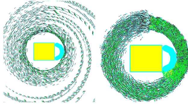
Fig. 3 Snapshots of the simulation of the circling of the Kabba in the Muslin Hajj peregrination. Besides the rectangular box (Kabba) lies the semi-circular wall (Hatim). The arrows represent the velocity of pedestrians. The snapshots are taken after 5 and 10 minutes.
